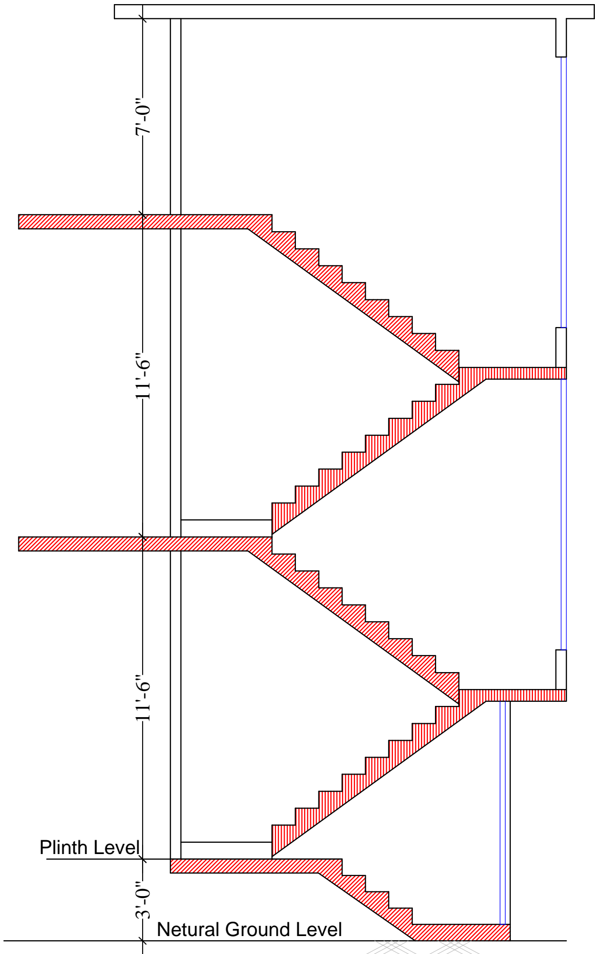
Stair Case Section
